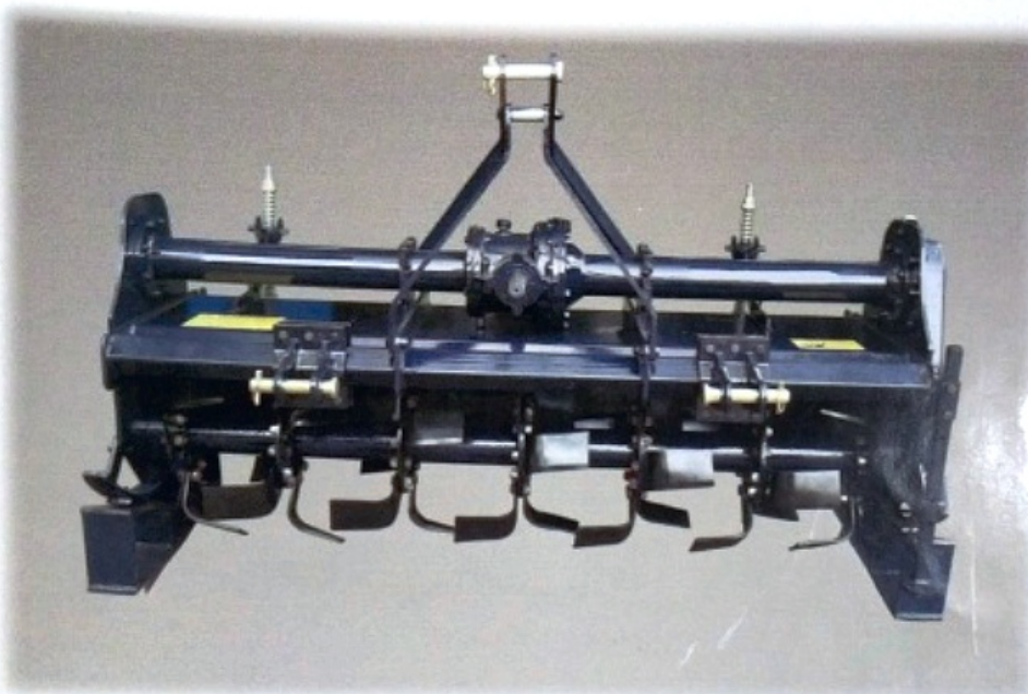
SINGLE SPEED 36 BLADE ROTOVATOR
