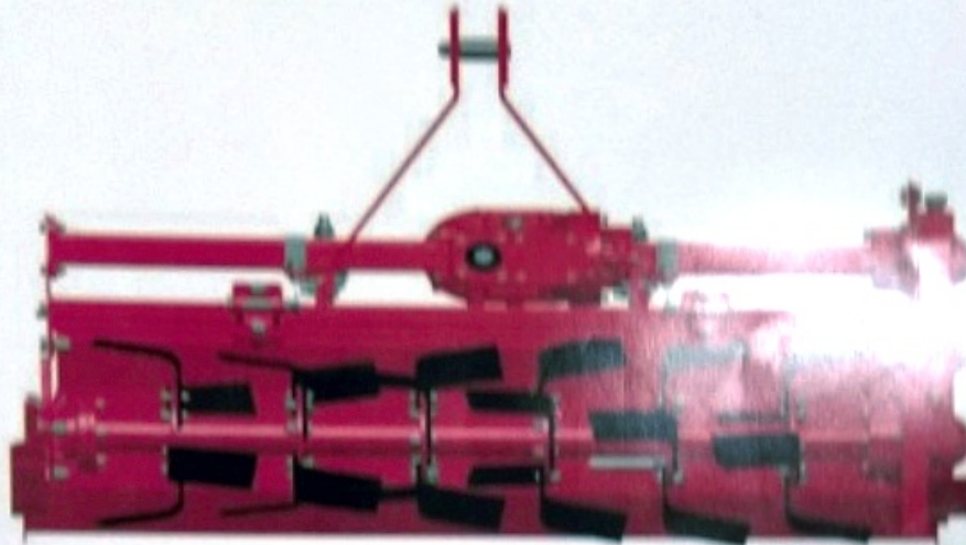
TAFE AGRISTAR 612MV – 24 BLADE MULTI SPEED ROTARY TILLER
