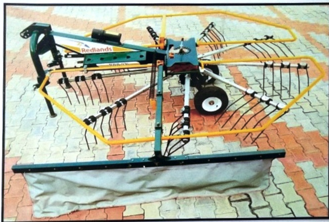
TRACTOR OPERATED ROTARY HAY RAKE RRR936
