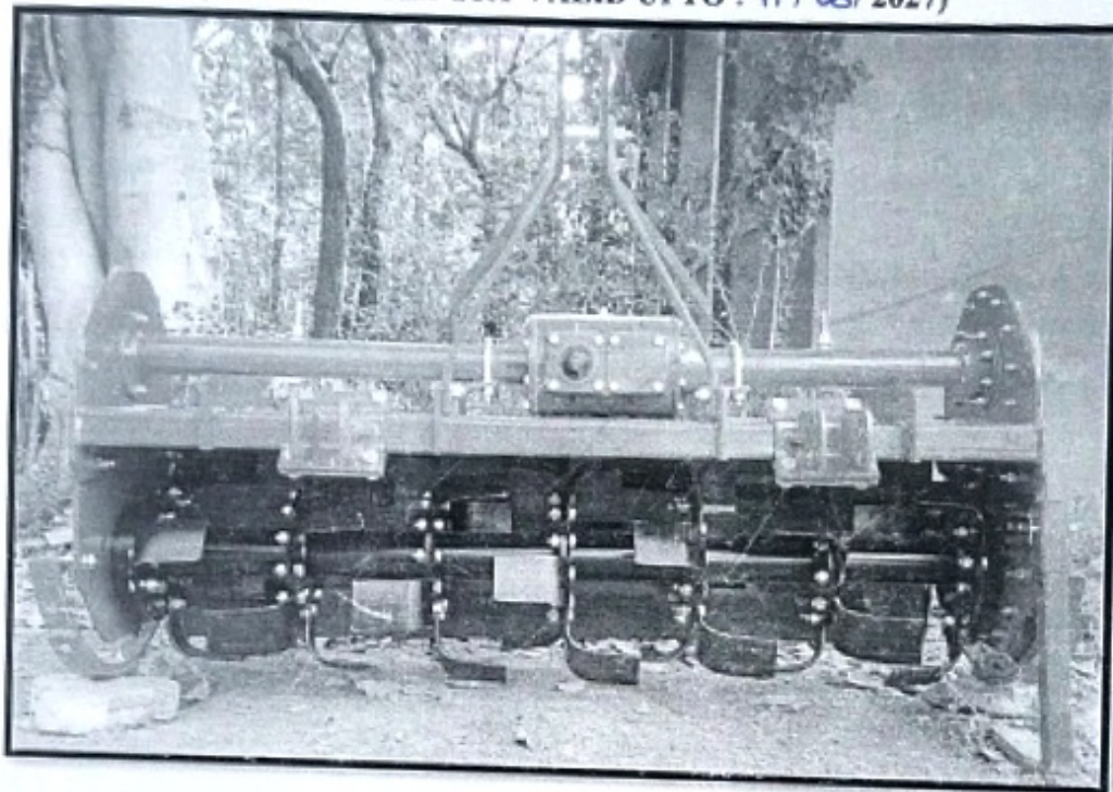
TAFE AGRISTAR 615VX – 36 BLADE MULTISPEED ROTARY TILLER
