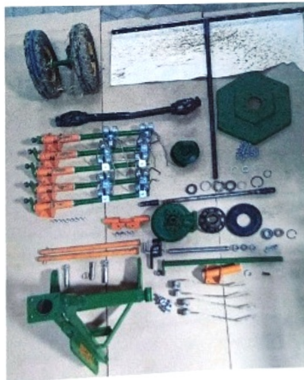
Fig.10: Dismantled view of the rotary hay rake
