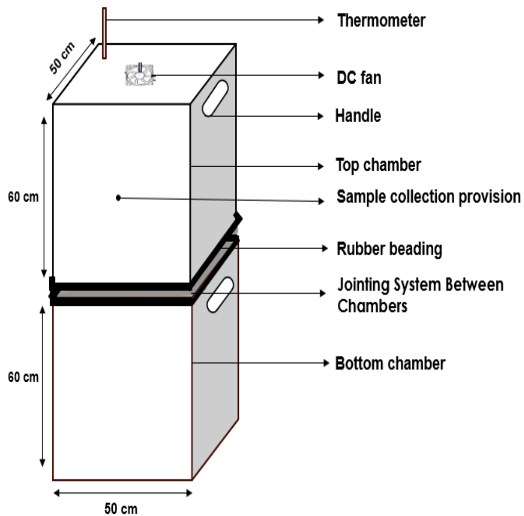
Fig: Technical illustration of the Greenhouse gas collection chamber
